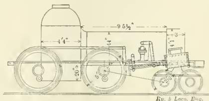
"SULLIVAN," FIRST ROGERS' ENGINE FOR ERIE RAILROAD.
